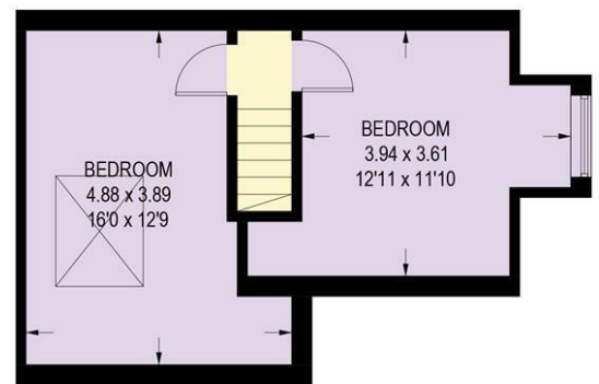
SECOND FLOOR = 32 SQ M / 344 SQ FT
